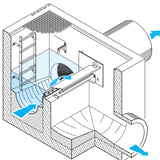
Bending Weir UFT-FluidBend
