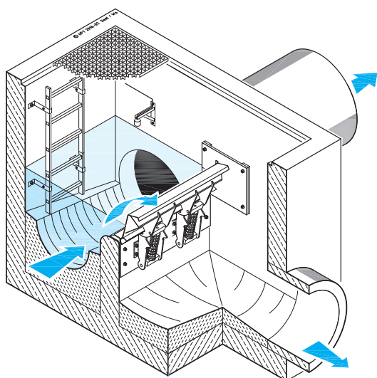
Spring-Loaded Weir UFT-FluidFlap
