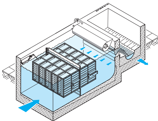
Cross Flow Lamella Settler UFT-FluidClearX
